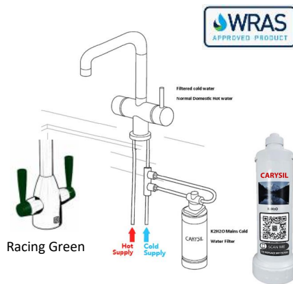
CBK2H2O Filter Kit –Optional Page 51
