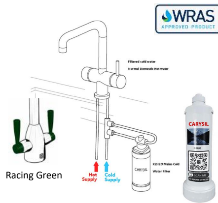
CBK2H2O Filter Kit- Optional Page 47
